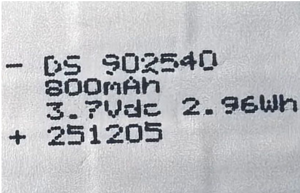
Figure 5 Battery label (电池标签)
