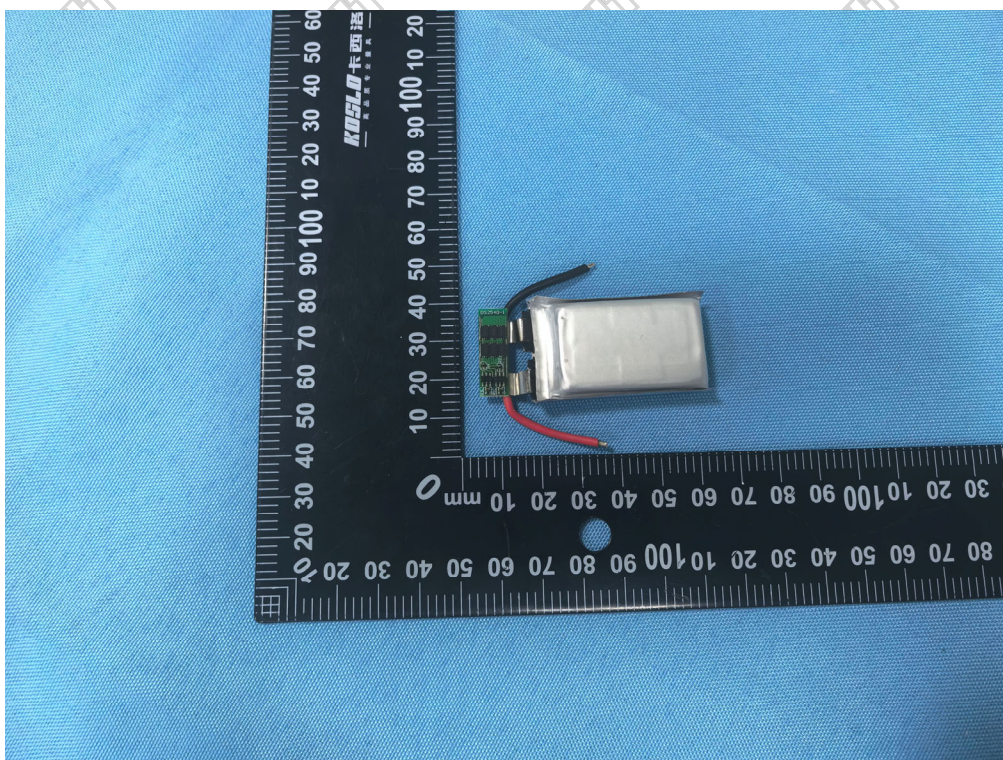
Figure 4 Battery internal view (电池内部图)
